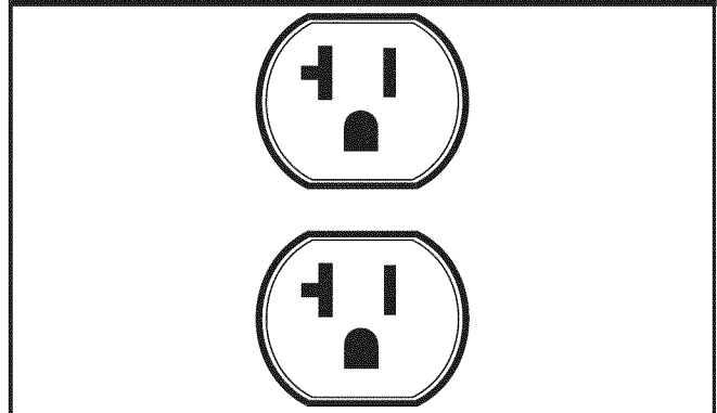
Figure 7 — 120 Volt, 20 Amp Duplex Receptacle
