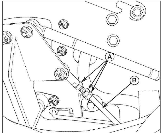
Figure 35. Return-to-Neutral Adjustment A. Jam Nuts B. Neutral Return Rod
