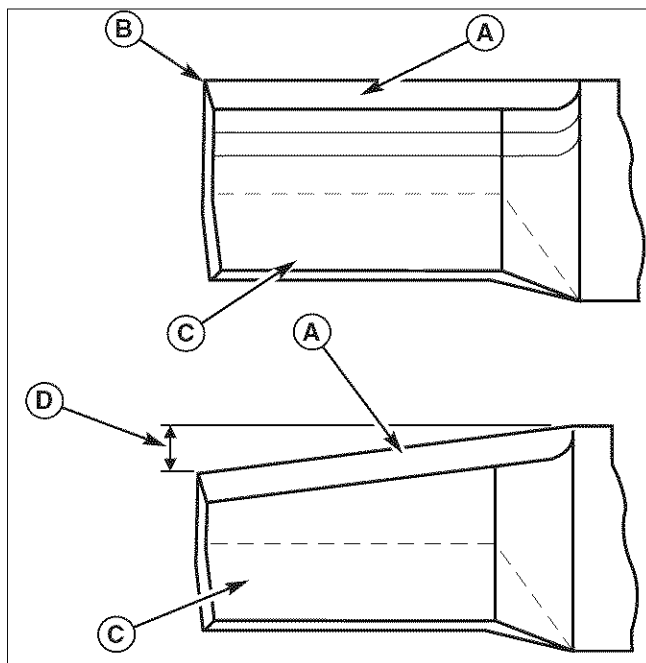
Figure 27. Inspecting the Mower Blade Tips
