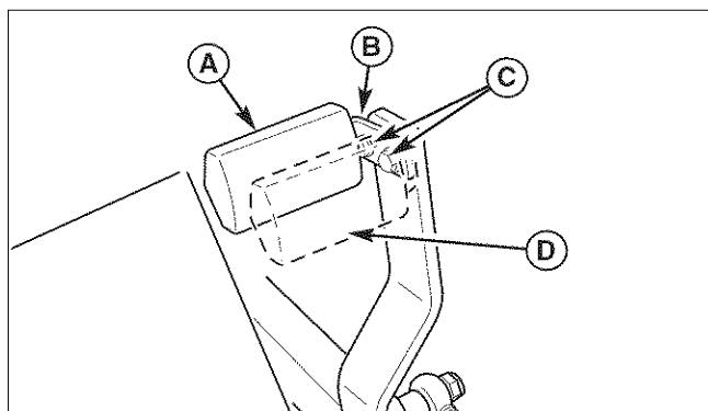
Figure 7. Foot Pedal Adjustment
