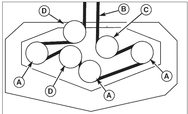
Figure 41. Mower PTO Belt Routing
