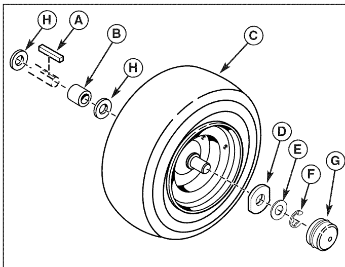
Figure 17. Rear Axle Hardware
