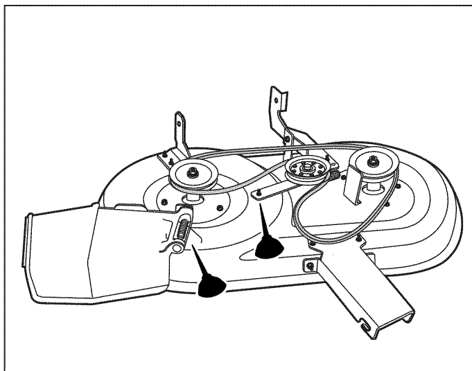
Figure 16. Lubricate Deck Linkage (38" shown)
