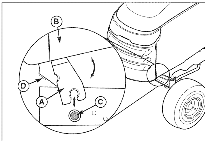
Figure 13. Hood Removal and Installation A. Hinge Post B. Hood C. Pivot Post D. Stop
