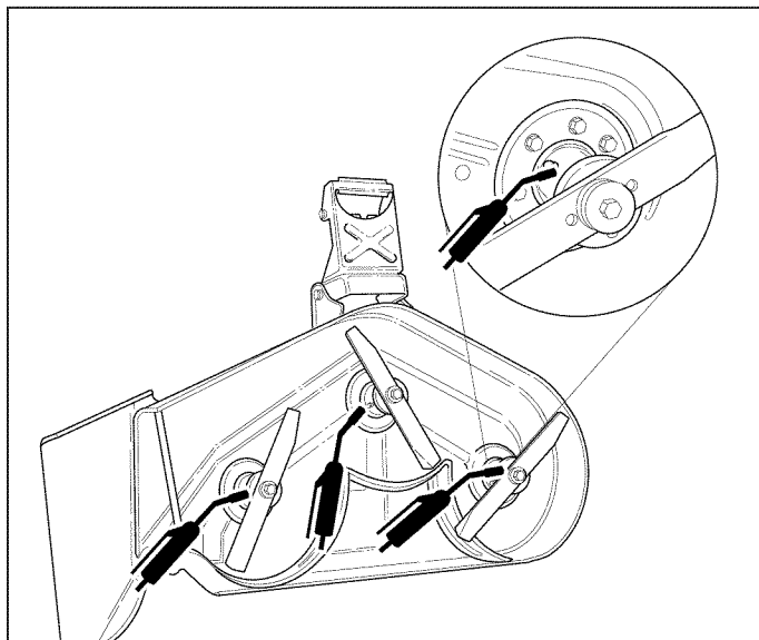
Figure 15. Arbor Lubrication Points
