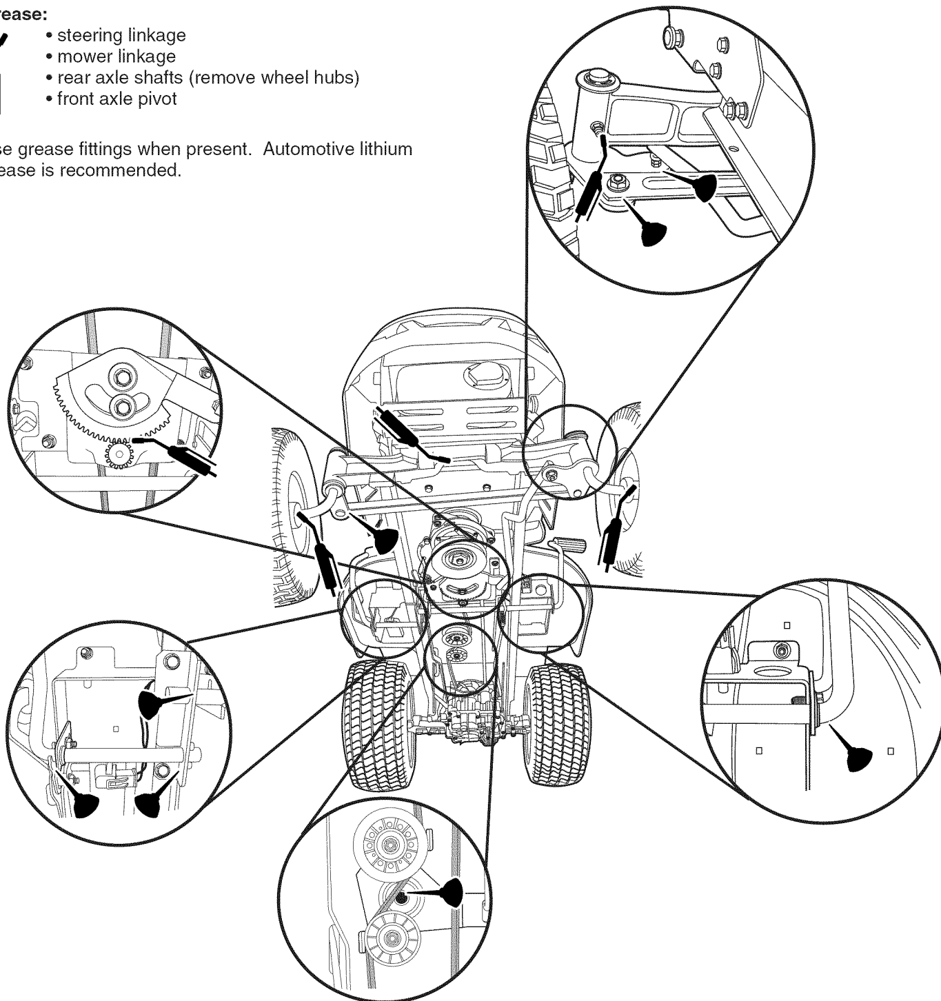
Figure 14. Lubricate Tractor
