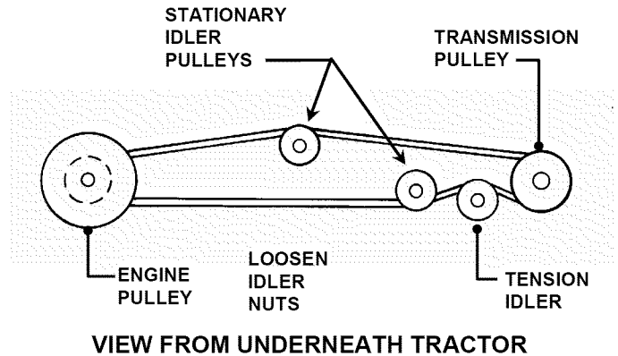
VIEW FROM UNDERNEATH TRACTOR
