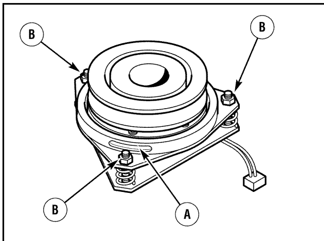
Figure 25: PTO clutch
