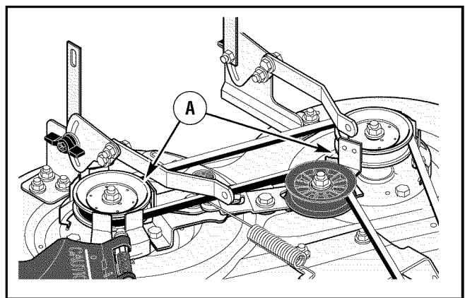
Figure 24: Blade brake
