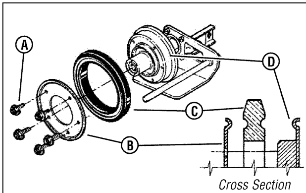
Figure 32: Replacing the driven disc rubber ring
