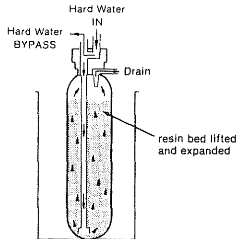
FIG. 10 WATER FLOW THROUGH THE SOFTENER IN BACKWASH
