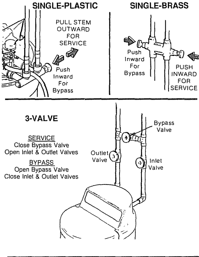
FIG. 16 BYPASS VALVES
