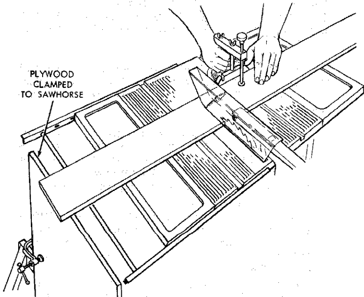
AUXILIARY FENCE
