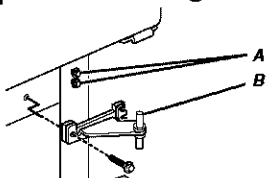
A. 5/16" Hex-Head Hinge Screws B. Center Hinge
