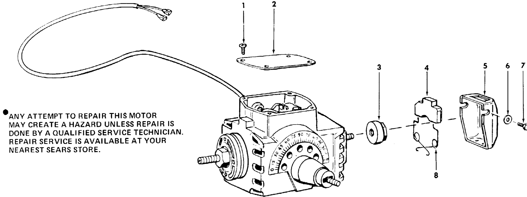
FIGURE 4 – 63605 MOTOR ASSEMBLY
