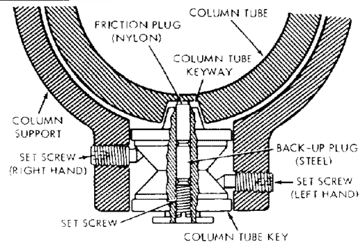
SECTIONAL VIEW LOOKING DOWN
