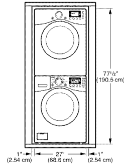
Required Dimensions for Installation With Stacking Kit
