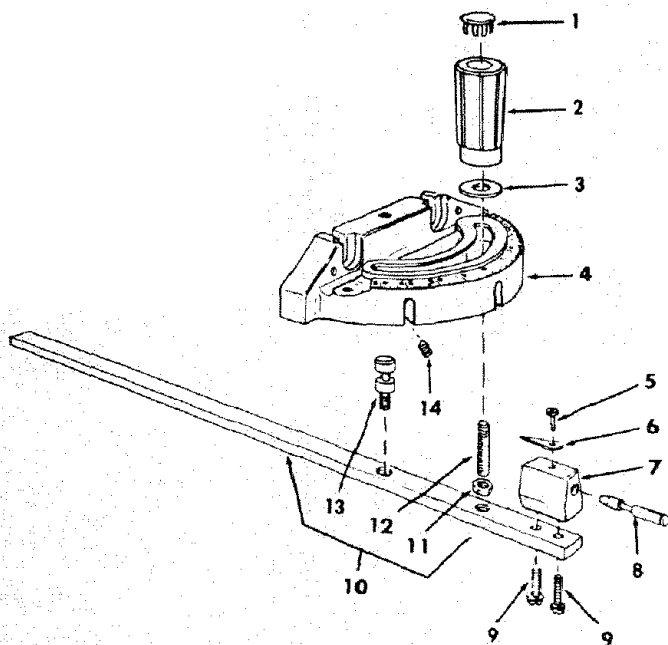
FIGURE 5 - 62704 MITER GAUGE ASSEMBLY
