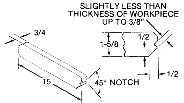
PUSH STICK
