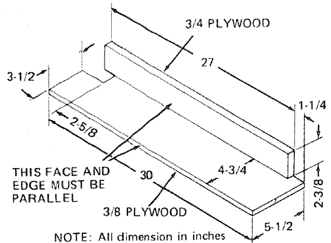
NOTE: All dimension in inches AUXILIARY FENCE/WORK SUPPORT
