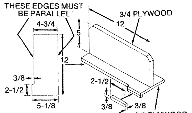
PUSH BLOCK
