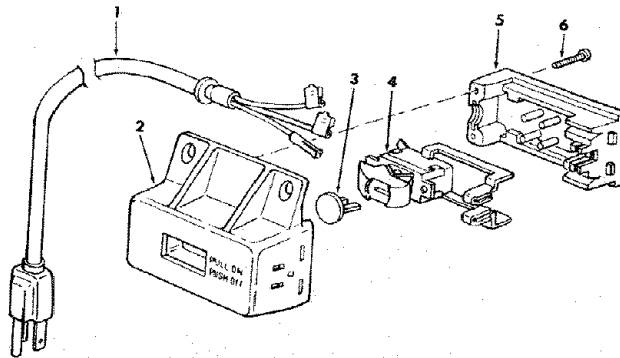
FIGURE 2 - ON/OFF POWER OUTLET 60381
