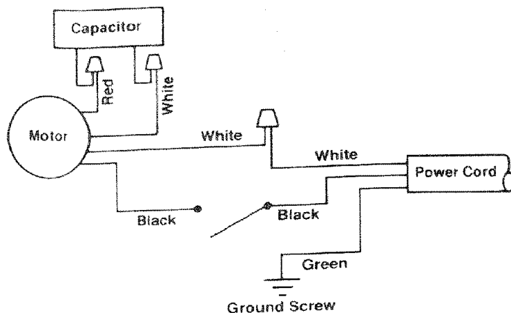
Wiring Diagram
