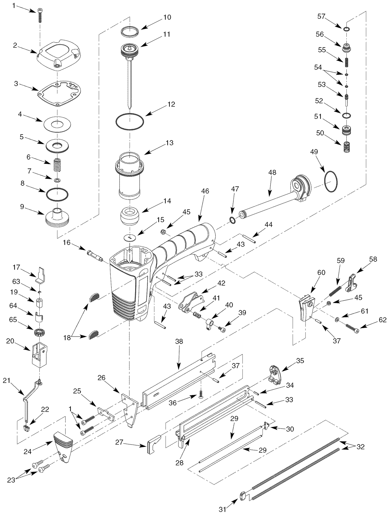
Figure 10 - Replacement Parts Illustration For Stapler
