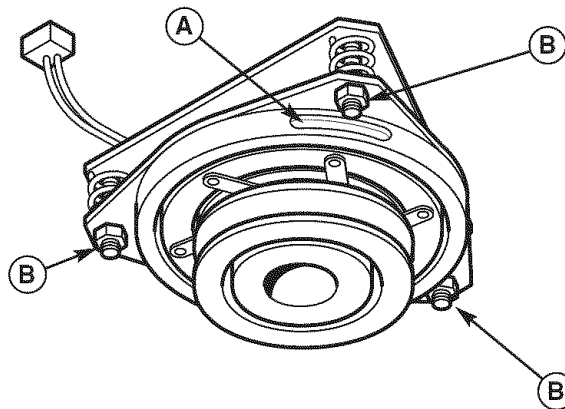
Figure 22. PTO Clutch Adjustment A. Adjustment Window (Qty. 3, one shown) B. Adjustment Nut
