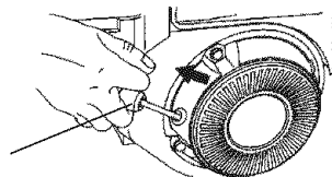
Rewind Starter
