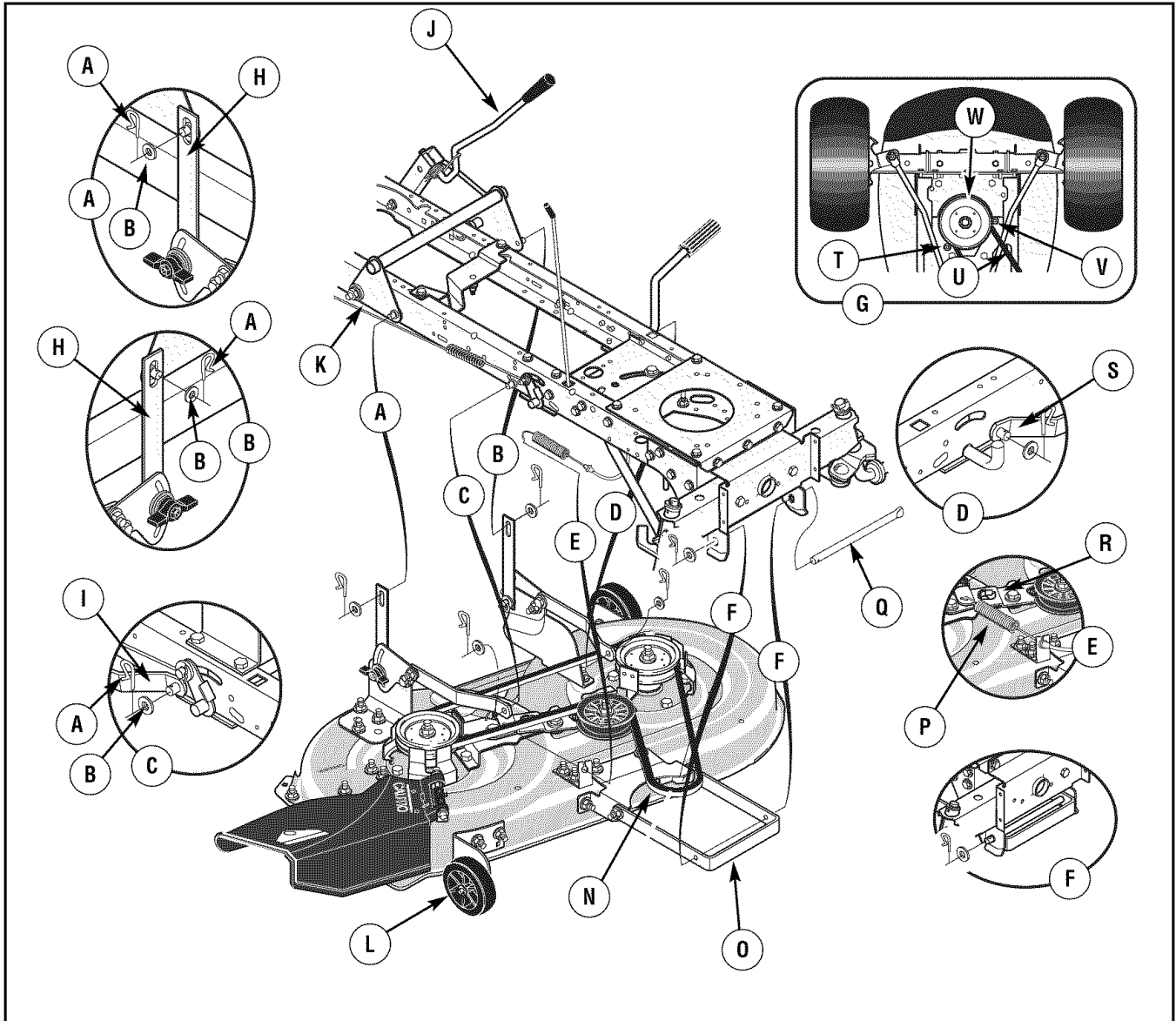
Figure 33: Mower deck assembly (42" models)
