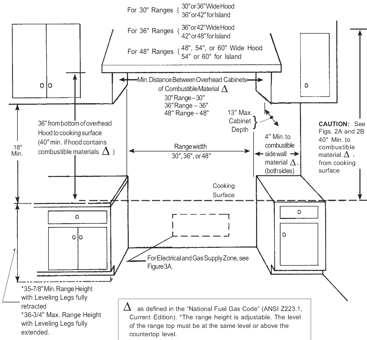
Figure 1: Cabinet Clearances
