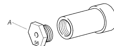
A. LP oven orifice spud stamped with "56"
