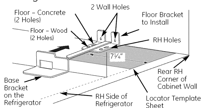
Figure 1 – Installation Overview
