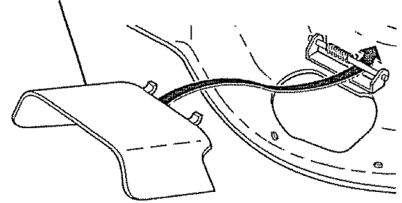
Discharge deflector
