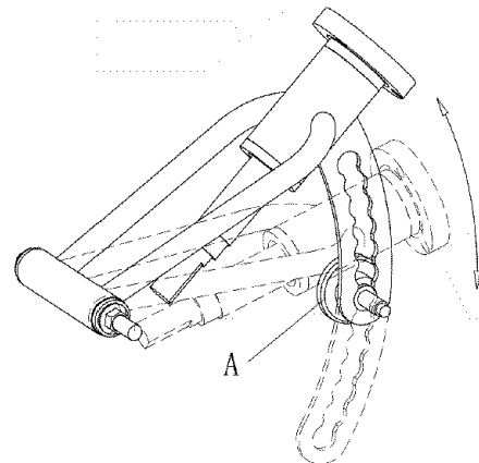
Steering Adjustment
