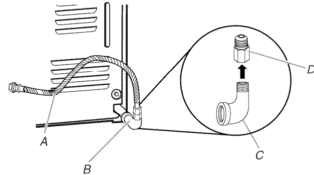
A. \frac{3}{8} " flexible gas connector
