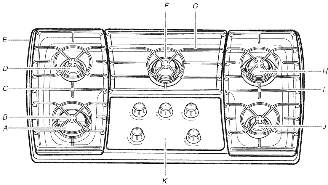
A. 17,000 Btu/h burner B. Surface burner cap C. Left surface burner grate D. 6,000 Btu/h burner (9,100 BTU burner on 30" [72.6 cm] models)
