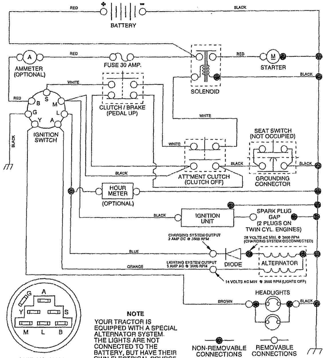
IGNITION SWITCH
