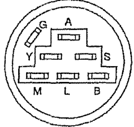
IGNITION SWITCH
