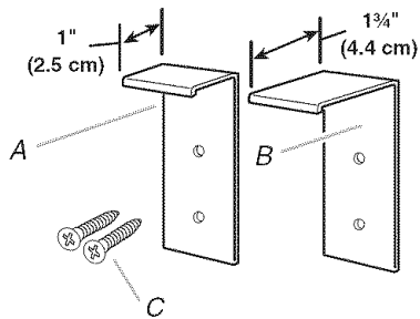
A. Anti-tip bracket - 1" (2.5 cm) B. Anti-tip bracket - 1 \frac{3}{4} " (4.4 cm) C. #10 x 2" Phillips head screws (2)
