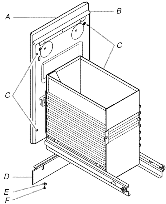
A. Custom panel B. 15" (38,1 cm) x ½" (13 mm) quarter-round C. Panel screw locations D. Toe guard E. Washer F. Toe guard screw
