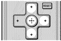
Pop-up menu
