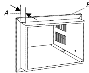
A. ½" (13 mm) extending into room B. Trim
