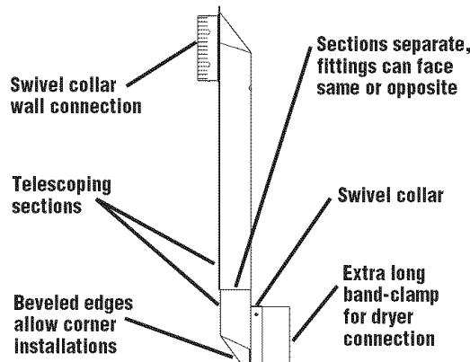
18"-29" : Part #4396011
