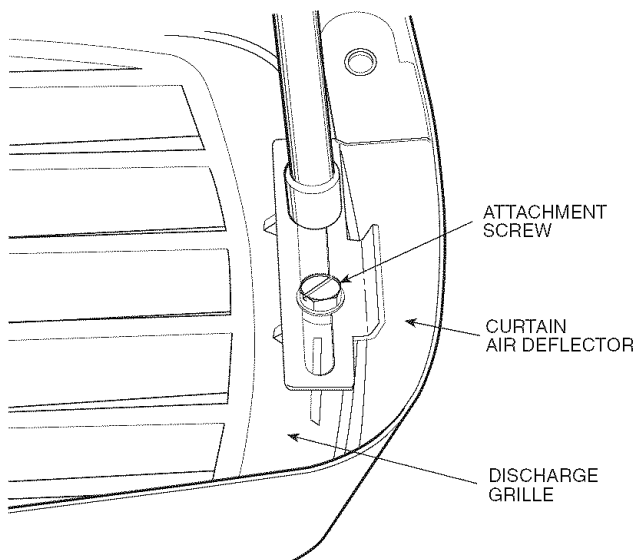
Fig. 4 — Attaching Discharge Grille to Curtain Deflector with 2 Screws
