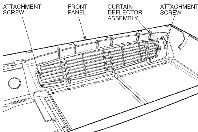
Fig. 5 — Attaching Curtain Deflector Assembly to Front Panel
