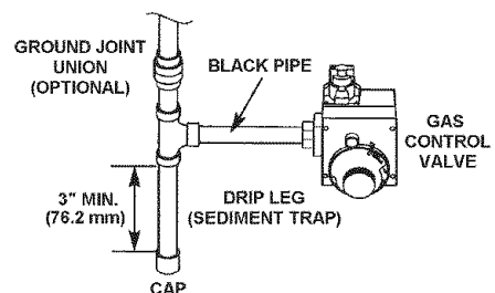
FIGURE 21. GAS PIPING WITH ALL BLACK IRON PIPE TO GAS CONTROL.
