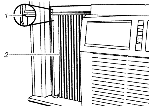
1. Hole for #8 x 3/4 in. round-head screw 2. Side curtain
