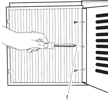
1. #8 x 3/8 in. pan-head screw
