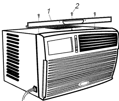
1. Top channel 2. #10 x \frac{3}{8} in. pan-head screw
