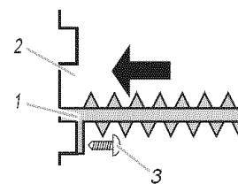
1. Side curtain against window channel 2. Window channel 3. #8 x 3/4 in. round-head screw
