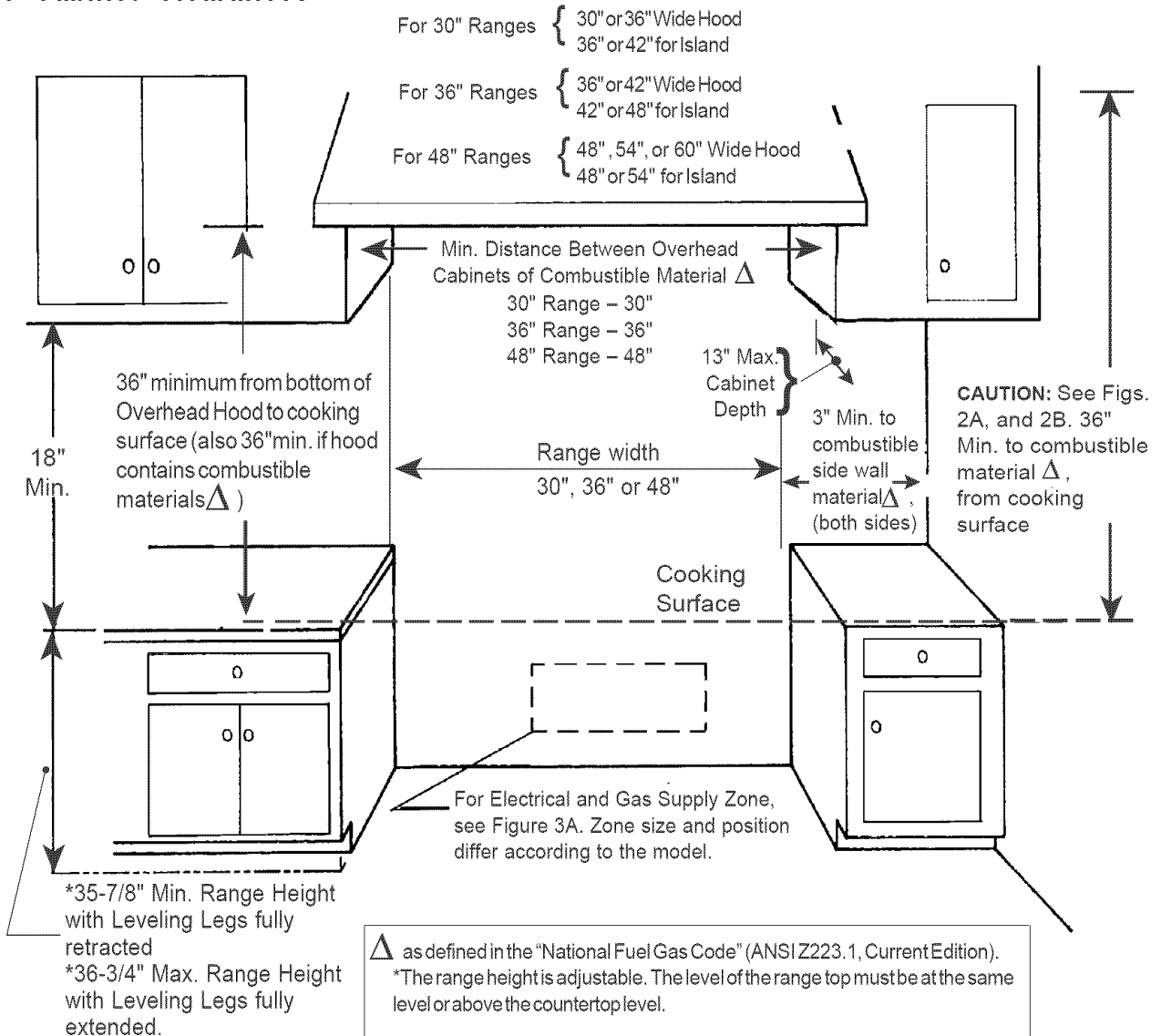
FIG. 1 Cabinet Clearances
