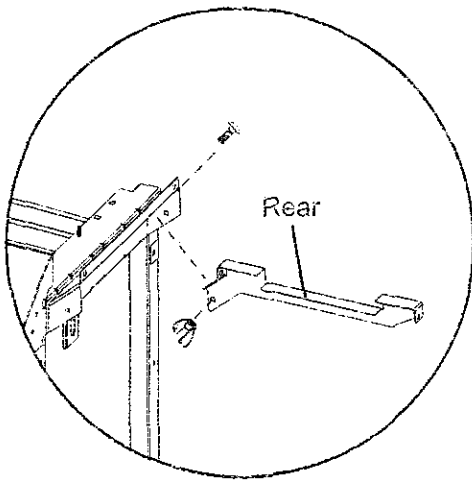
Shelf Brackets fit "inside" mounting bracket.
