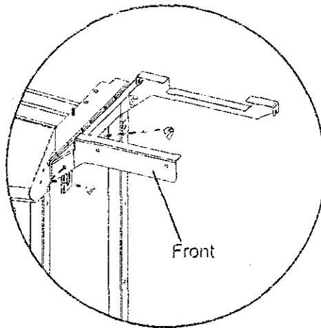
Attach Shelf Brackets with (2) 1/4-20 x 1/2" carriage bolts and (2) tapered wing nuts.
