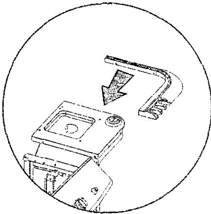
Attach Shelf Trim by, First sliding plastic tab on shelf trim into slot on burner base as shown. Then fix trim to burner base with (3) 1/4-20 x 1/2" carriage bolts and (3) tapered wing nuts.
