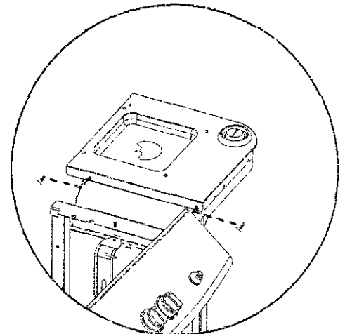
Attach Burner Base with (2) 1/4-20 x 1/2" carriage bolts and (2) tapered wing nuts.
