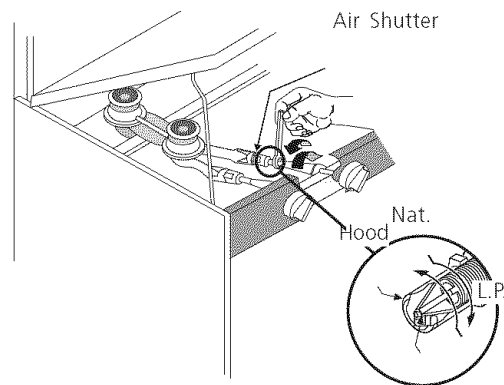
Top Burner Adjustment Figure 9
