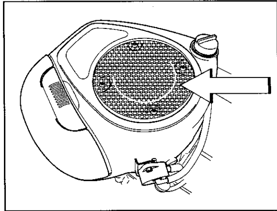
Check and clean the cooling air intake
