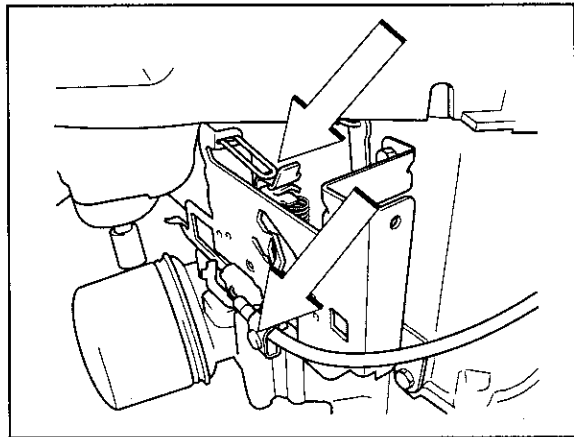
Adjusting the throttle cable
