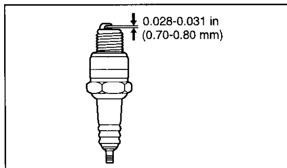
Measure the electrode gap
