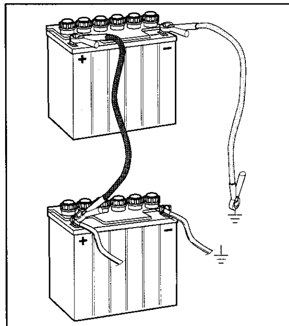
Jumper cables connection
