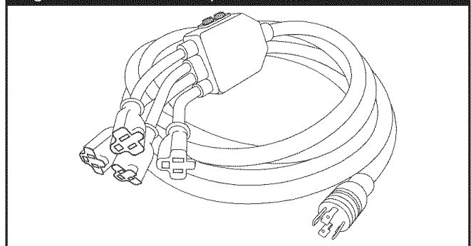
Figure 9 — Generator Adapter Cord Set
