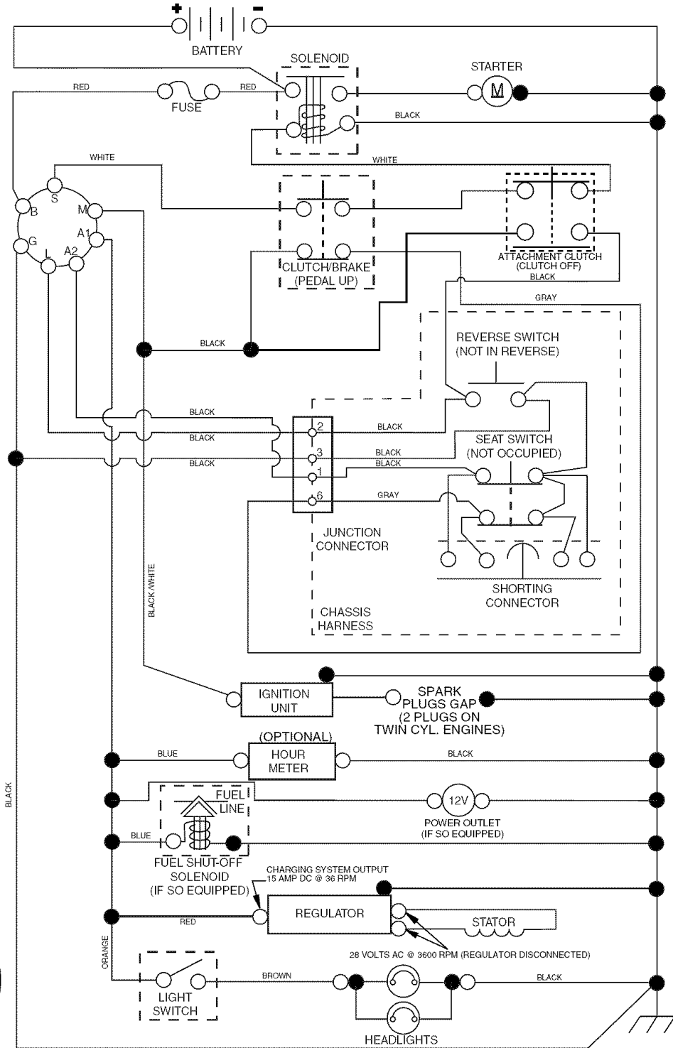
NON-REMOVABLE CONNECTIONS
