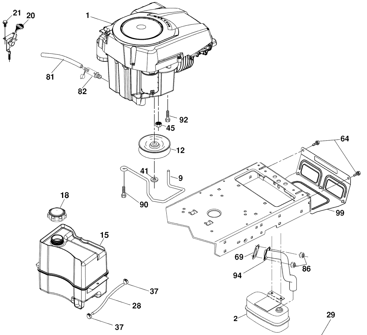
SPARK ARRESTER KIT
