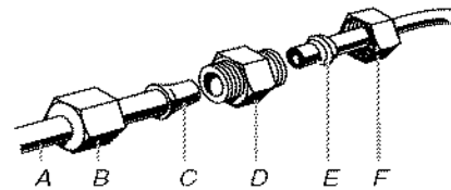
A. Water tubing B. Nut (provided) C. Bulb D. Coupling (provided) E. Ferrule (purchased) F. Nut (purchased)
