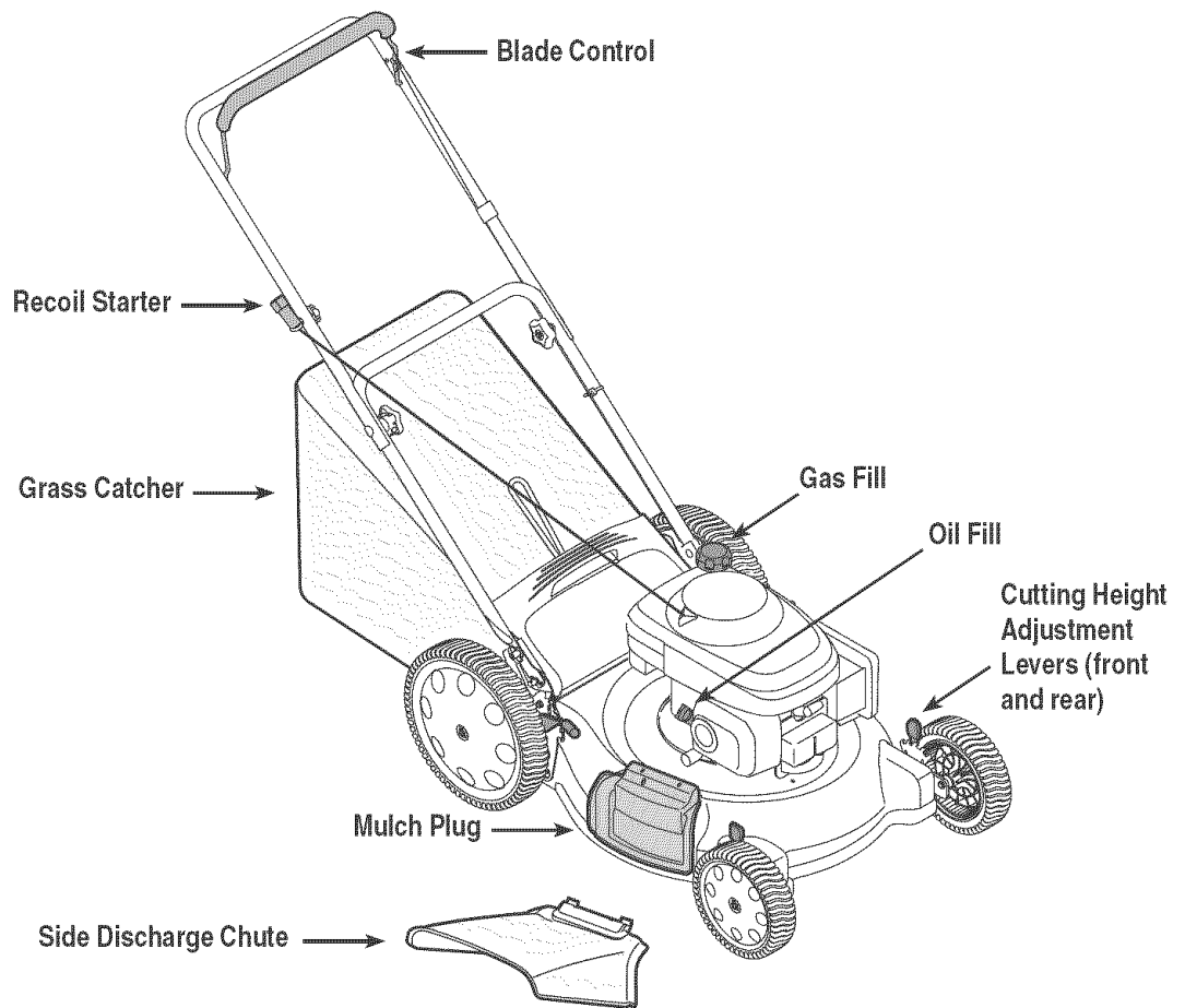
Figure 4-1: The major parts on the lawn mower.
