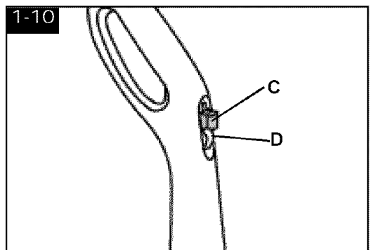
Pull switch lock (C) above ON/ OFF switch (D) straight out. Dispose of switch lock. If switch lock has come off during assembly, make sure switch is in OFF position (down) before plugging into electrical outlet.
