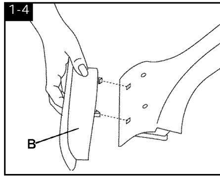
Snap tabs on hose holder (B) into holes on handle section.
