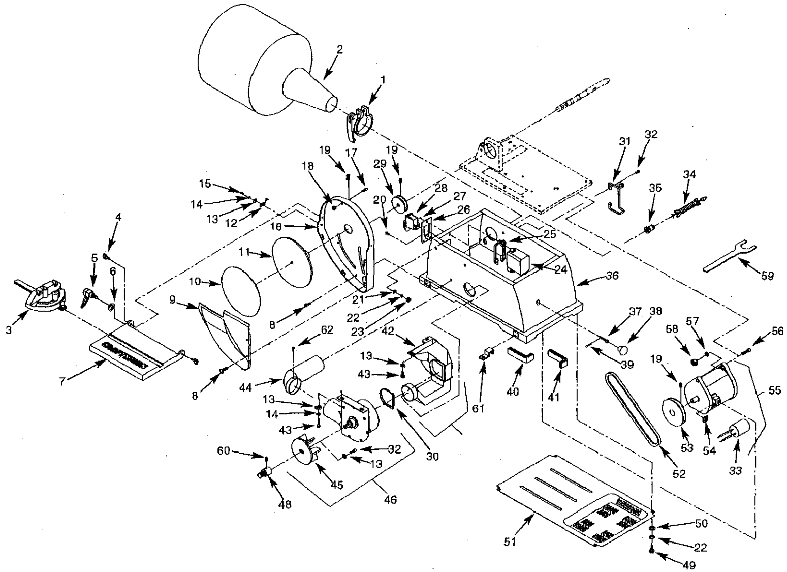
Figure 20 - Replacement Parts Illustration for Motor and Disc
