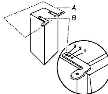
A. Countertop B. Retaining bracket
