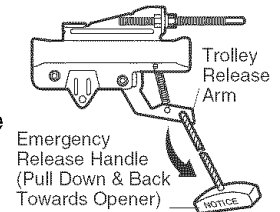
LOCKOUT POSITION
