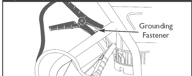
Figure 7 — Jumper Cable Connections
