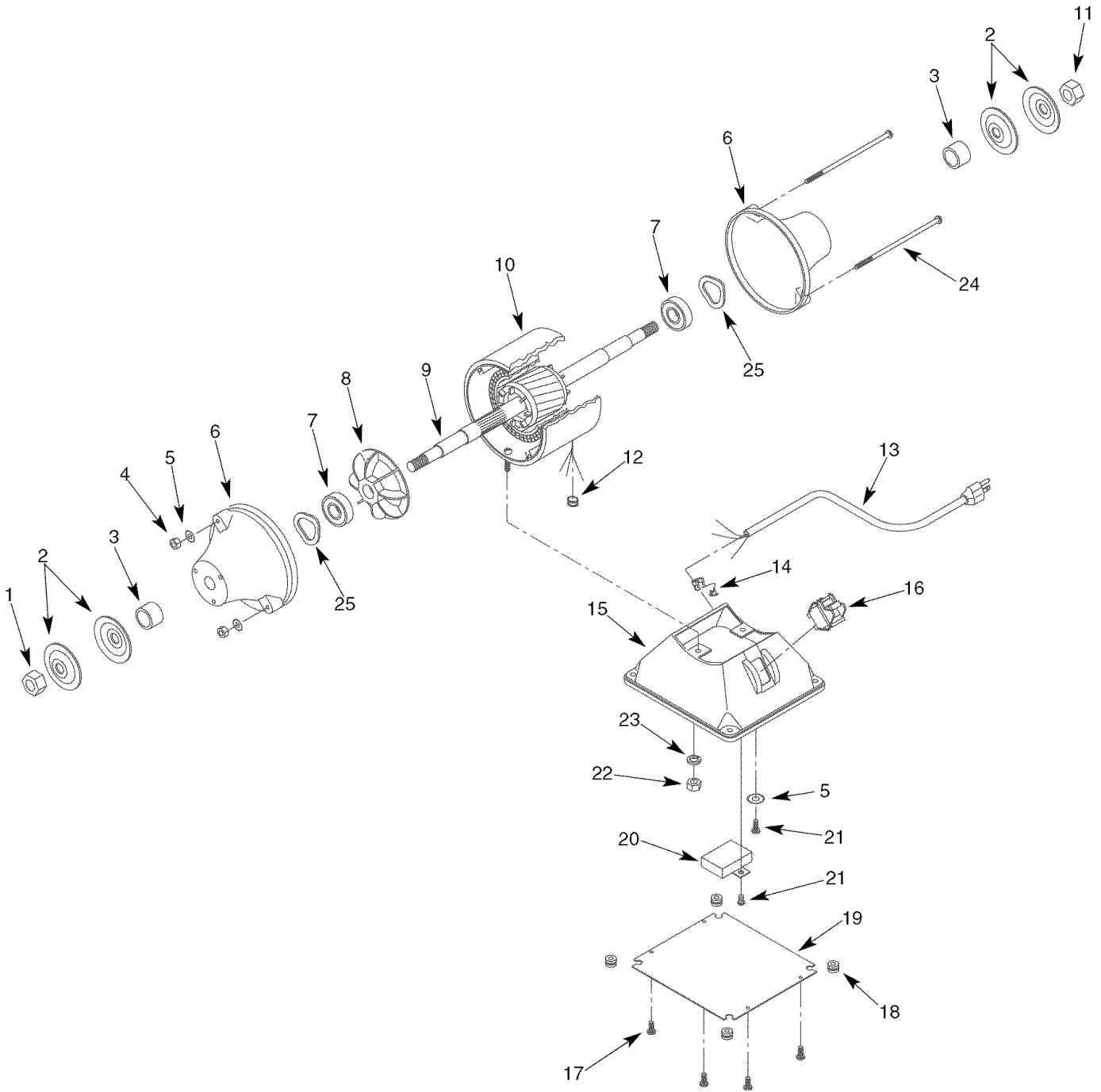
Figure 3 - Replacement Parts Illustration for 6" Buffer
