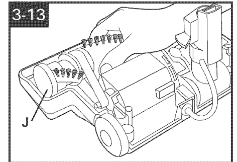
Stretch belt back and attach to motor pulley. Hold opposite end of agitated brush roll in place. Push belt end forward, rotating end plate (J) until it slides into place. Turn agitator, making sure it rotates freely.
