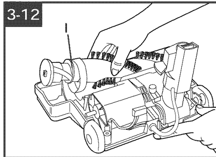
Lift up end of agitated brush roll. Remove old belt from agitated pulley (I) and replace with new belt. Lettering on belt must be visible.
