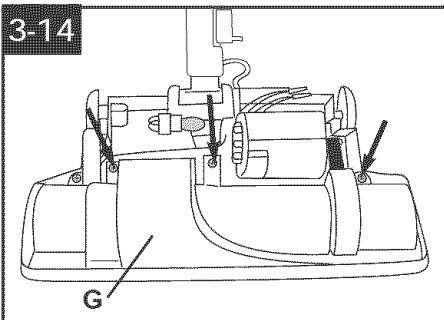
Replace brush roll cover (G) over agitator brush roll. Replace 3 short screws.
