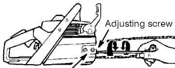
Chain Brake Nuts
