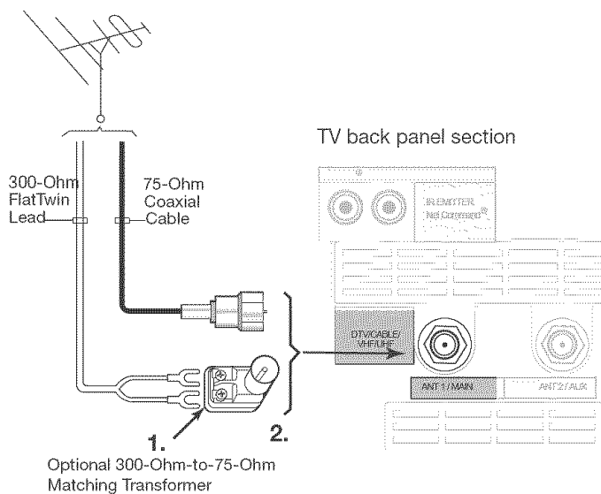
Figure 3. Connecting a Single Antenna
